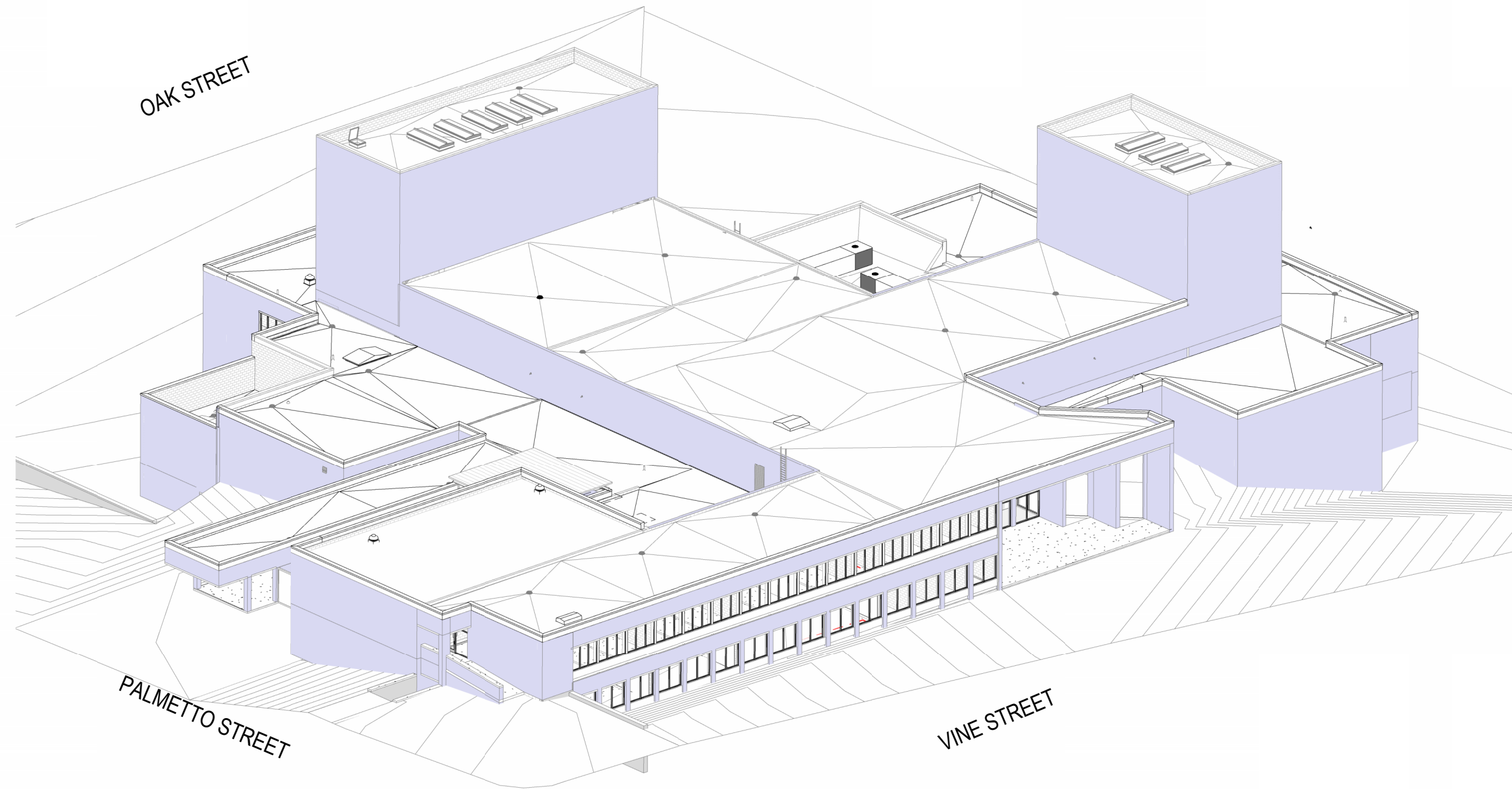
NORTH EAST CORNER
