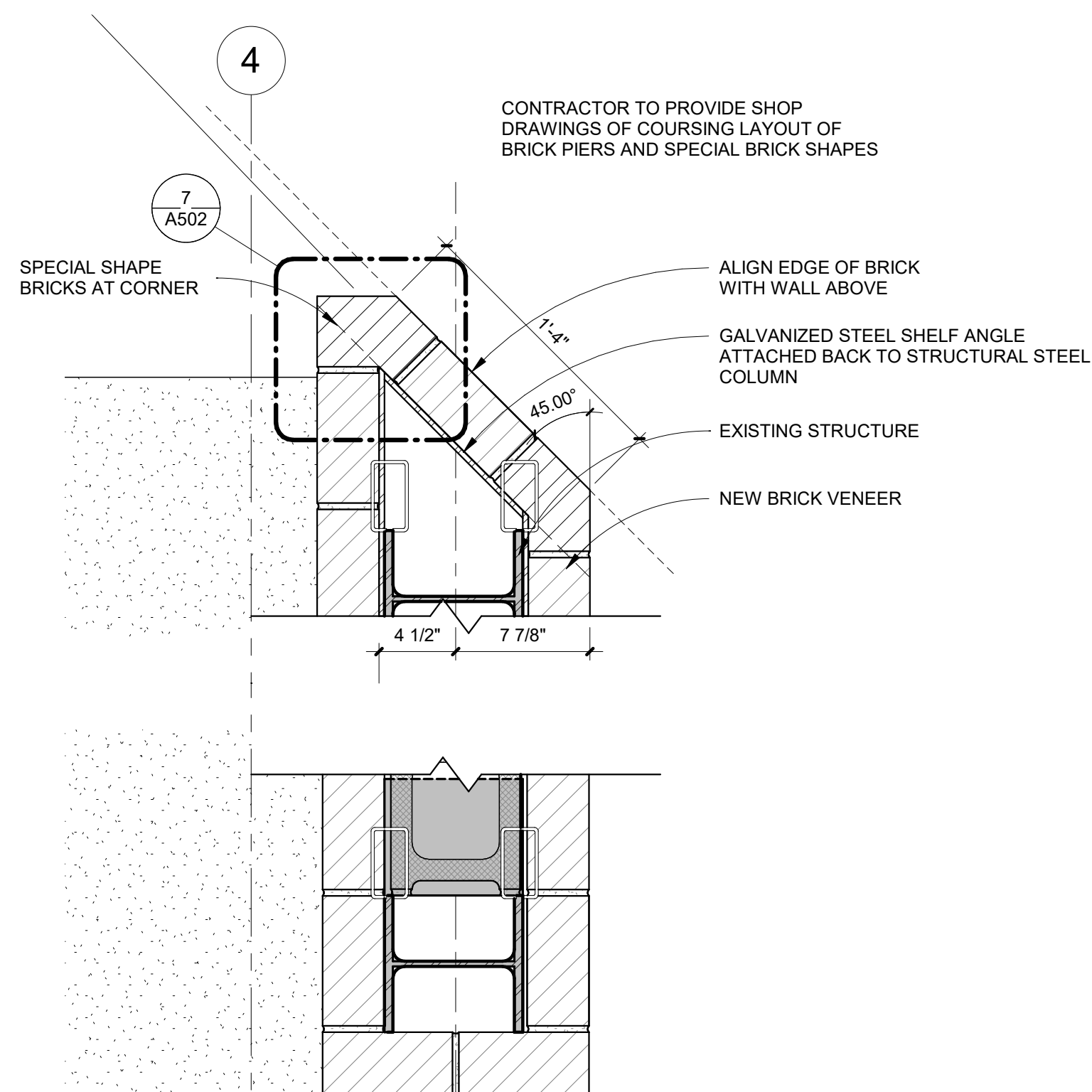
PLAN DETAIL - BRICK PIER @ NORTH ENTRY
