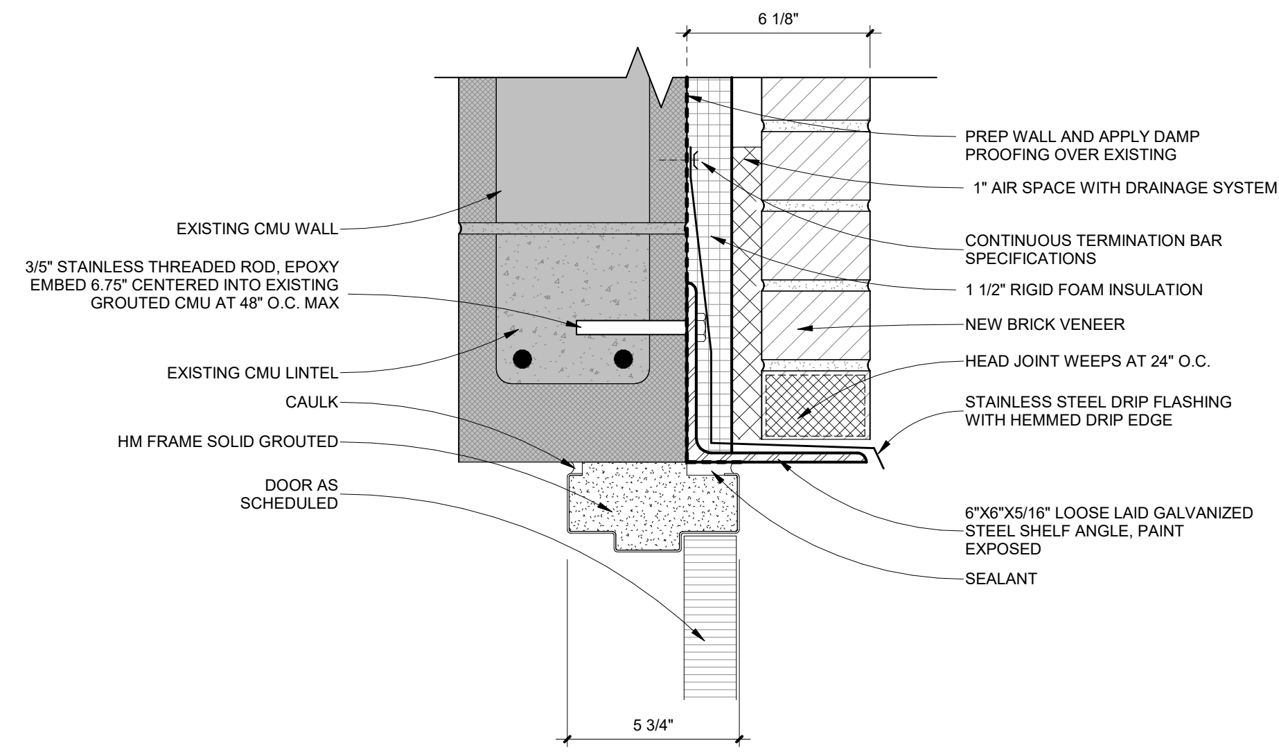
DETAIL@ HOLLOW METAL DOOR HEAD
