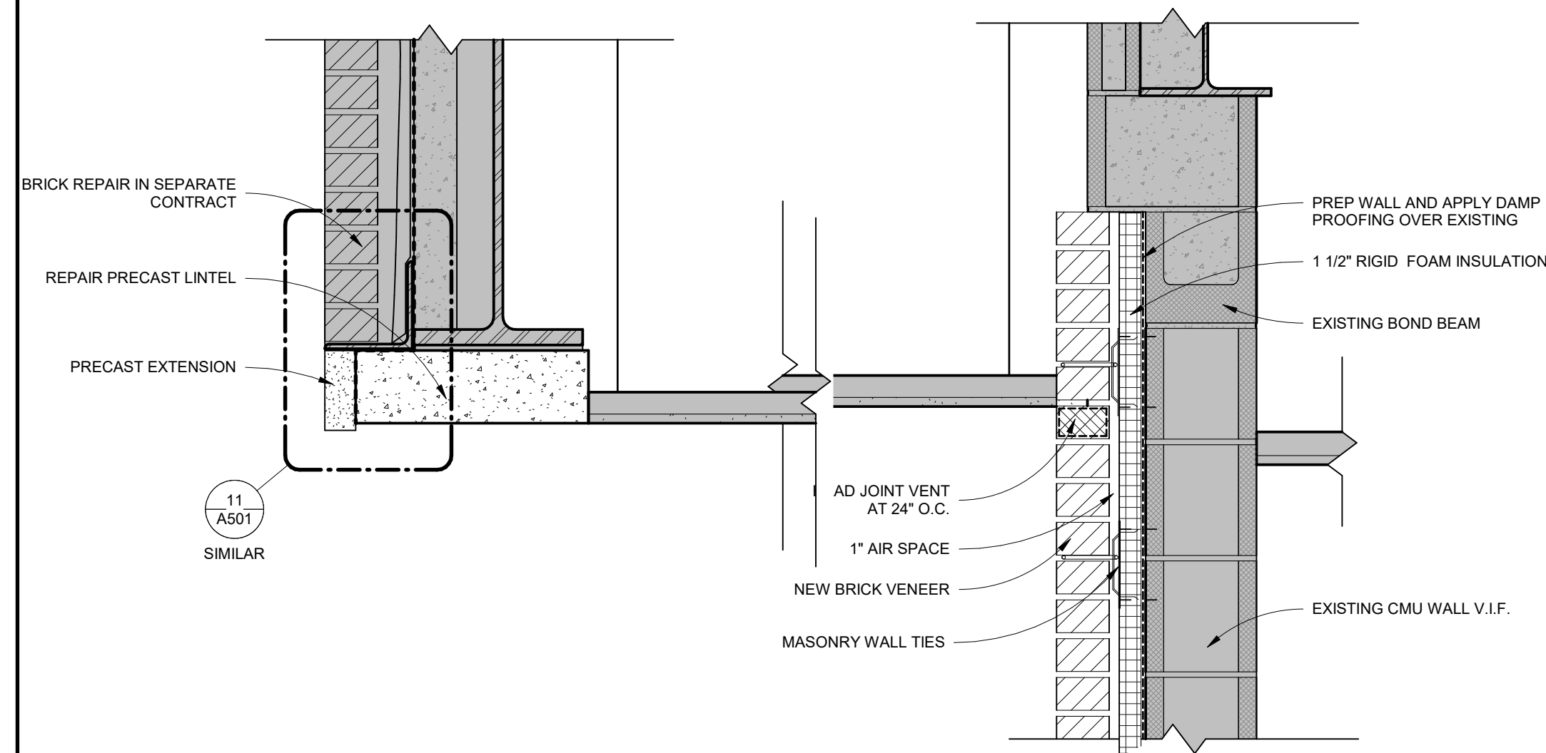
WALL SECTION @ NORTH ENTRY
