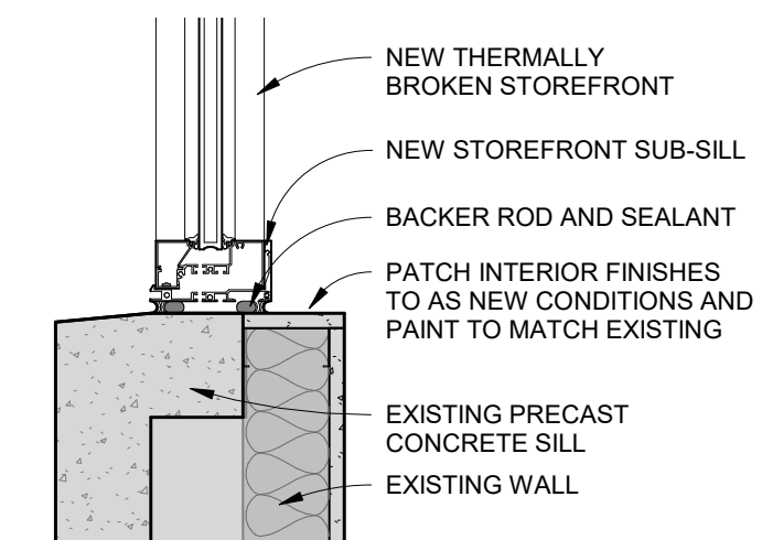
DETAIL@ STOREFRONT SILL
