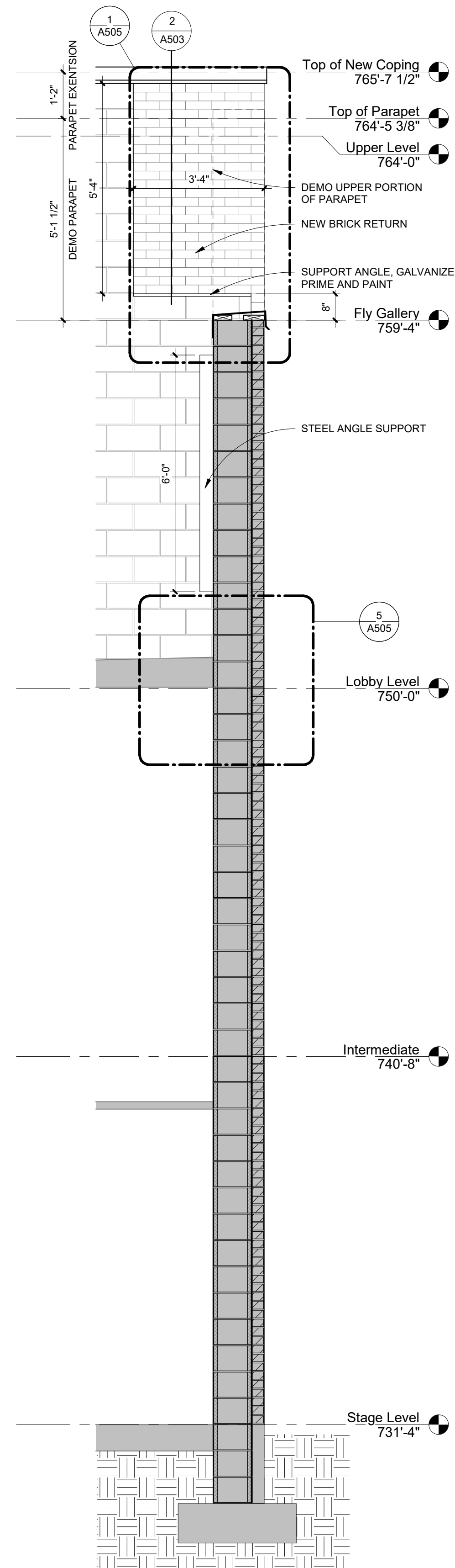
TYPICAL WALL SECTION @ MECHANICAL WELL
