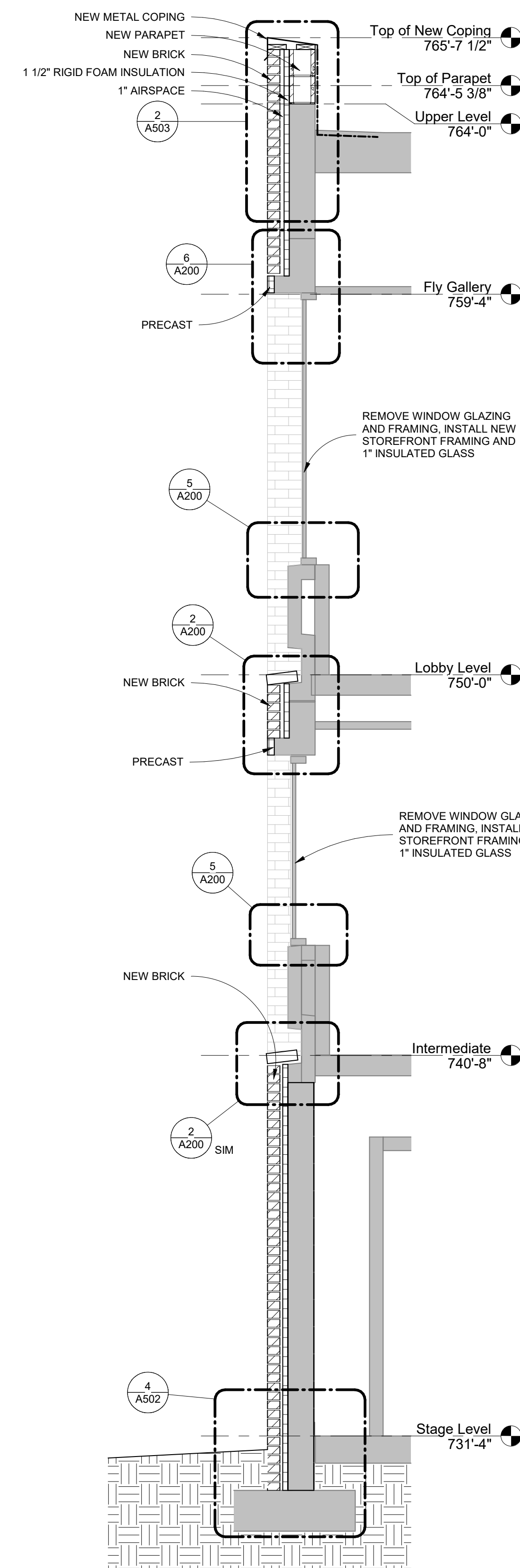
TYPICAL WALL SECTION @ STOREFRONT
